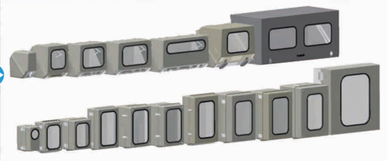
INTERTEC offers the world's broadest range and most flexible service for outdoor two-part GRP enclosures. Standard styles of enclosures include diagonally opening DIABOX enclosures (top) and MULTIBOX or MINIBOX enclosures (bottom - MINIBOX shown at left end).
